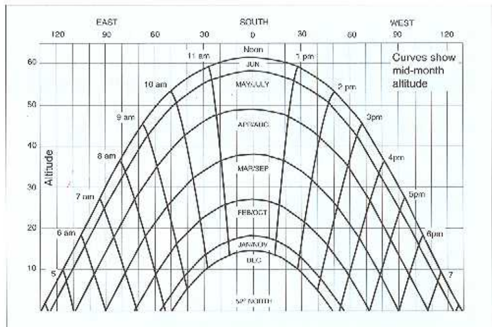
Figure 1 Sun-path diagram shows position of sun throughout year and enables designer to plot shadows from obstructions.
