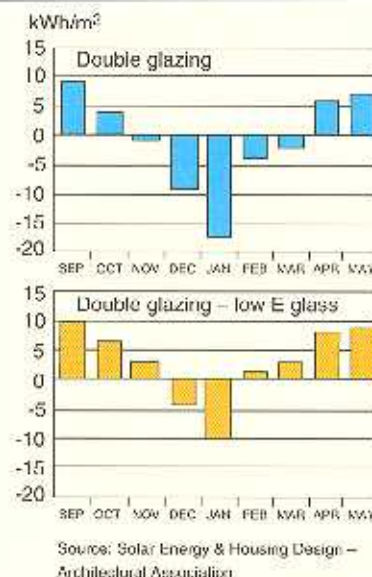
Figure 4 Comparison of the energy balance of south facing double glazing with and without low emissivity glass (Sheffield).
